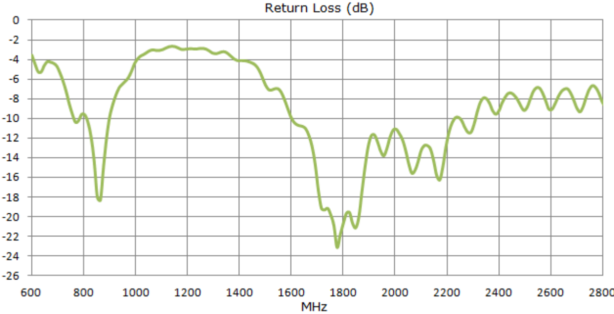
Figure 3. Return Loss of G30 Antenna on 30x30cm metal
