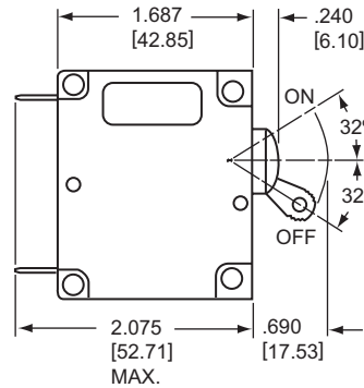
Single Pole Protector
