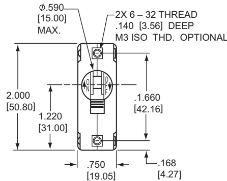
Single Pole Mounting Detail
