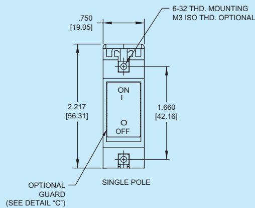
Panel Mounting Detail
