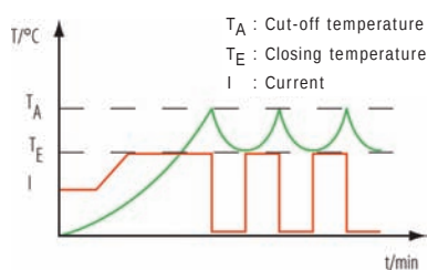
Functional diagram
