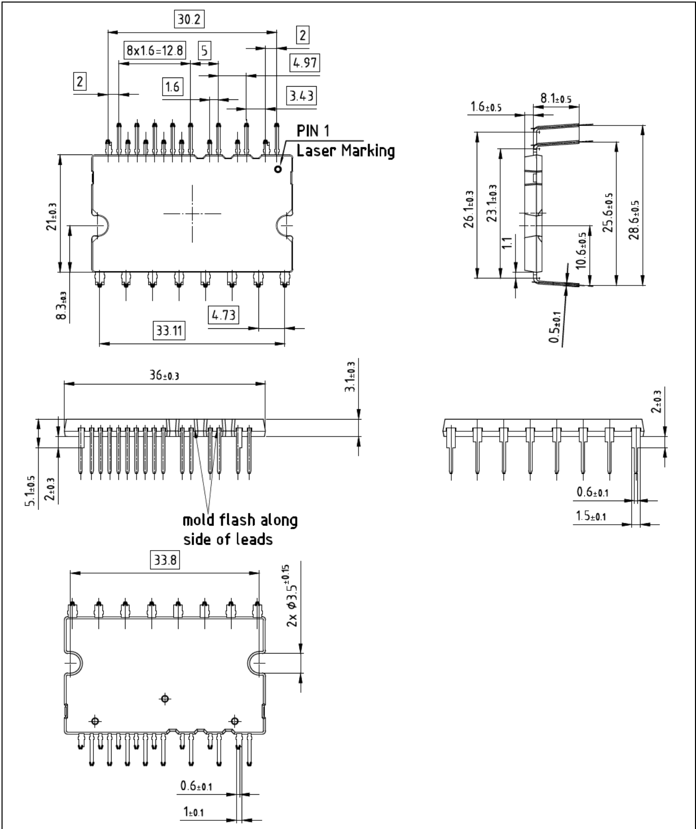
Figure 13 IM06B20AC1
