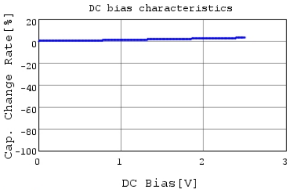
ECASD40E477M4R5KA0 C-DC bias capchange, 25.0
