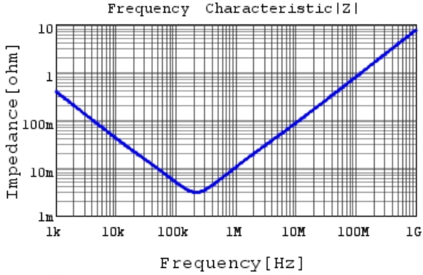
ECASD40E477M4R5KA0 |Z| DC0V, 25degC
