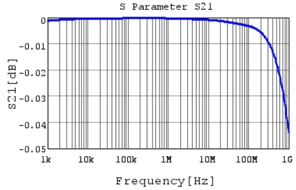
ECASD40E477M4R5KA0 S21 DC0V, 25degC
