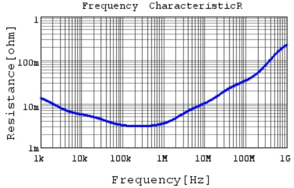
ECASD40E477M4R5KA0 R DC0V, 25degC
