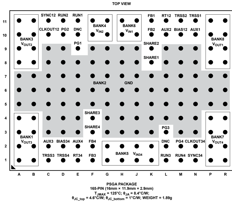
Figure 5. Pinout Configuration
