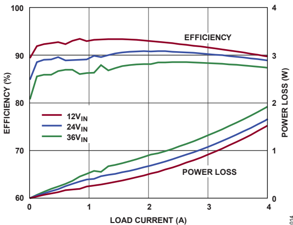
Figure 14. Efficiency vs. Power Loss, V_{OUT} = 3.3V , BIAS = 5V , Burst Mode Operation
