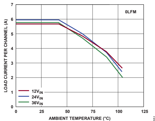
Figure 51. Dual Channel Derating, V_{OUT} = 5V CH1/CH3 ON, CH2/CH4 OFF, BIAS = 5V, DC2820A-B Demo Board, T_J = 120^{\circ}C , Burst Mode Operation
