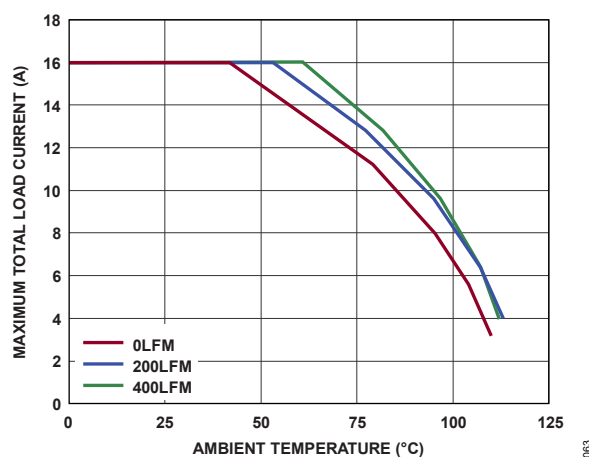
Figure 63. 12V IN to 5V OUT Derating with Airflow
