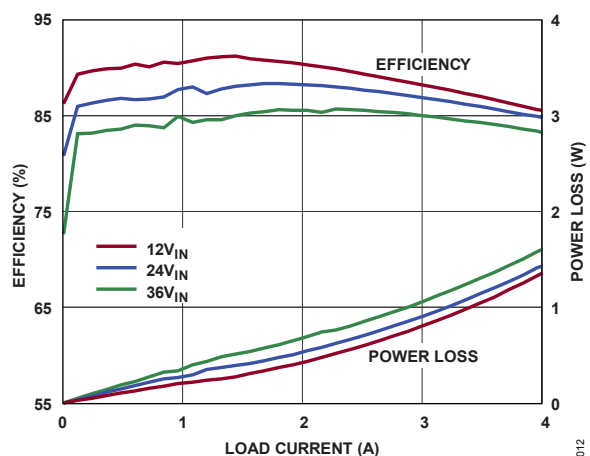
Figure 12. Efficiency vs. Power Loss, V_{OUT} = 2V , BIAS = 5V , Burst Mode Operation
