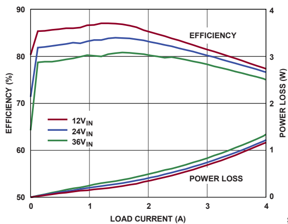
Figure 8. Efficiency vs. Power Loss, V_{OUT} = 1\text{V} , \text{BIAS} = 5\text{V} , Burst Mode Operation
