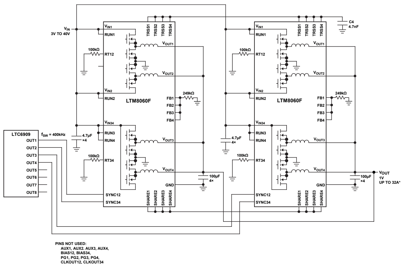
Figure 73. Two LTM8060F are Paralleled to Supply 1V at 32A Output with 45° Phase-Shift Interleaving Through All Eight Channels
