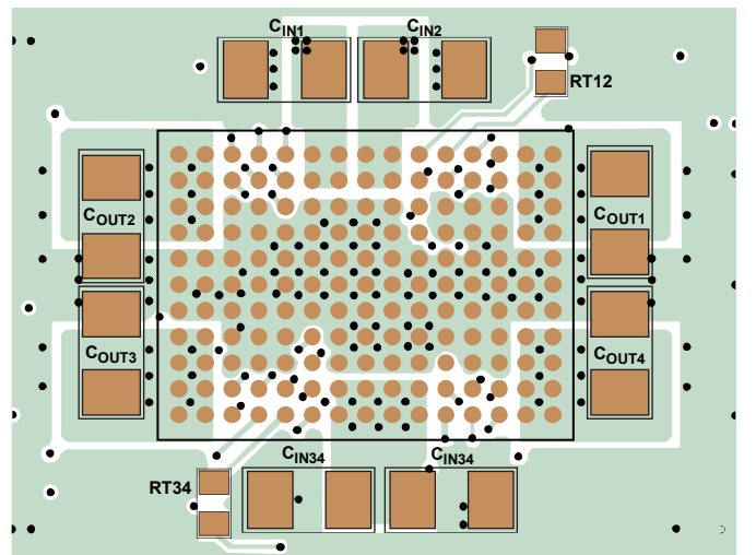
Figure 67. Layout Showing Suggested External Components, GND Plane, and Thermal Vias
