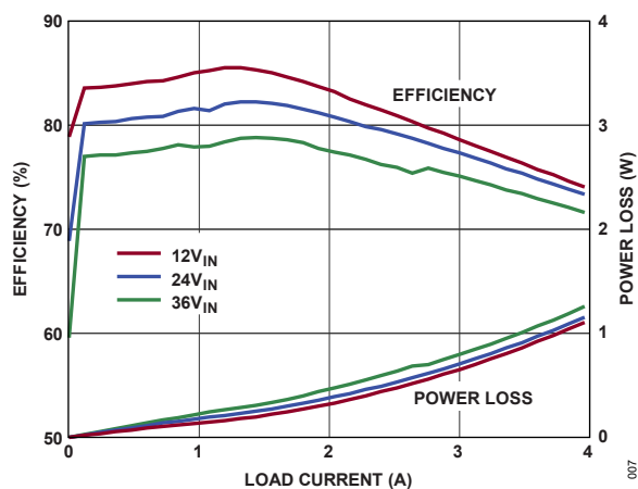
Figure 7. Efficiency vs. Power Loss, V_{OUT} = 0.8\text{V} , \text{BIAS} = 5\text{V} , Burst Mode Operation
