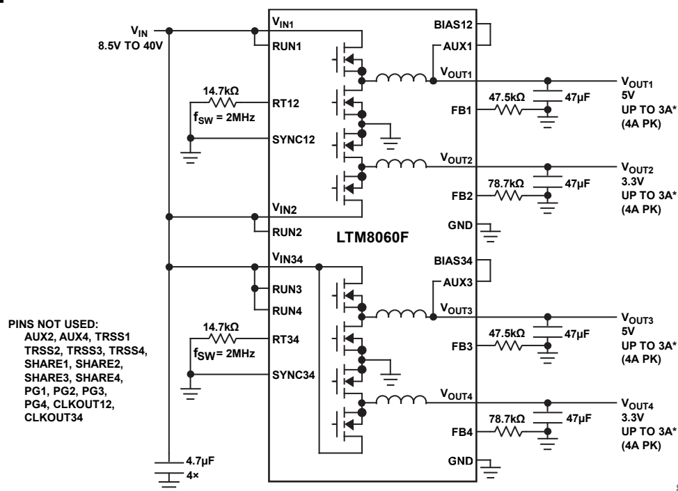
Figure 69. 8.5V to 40V Input to 5V at 3A (4A Peak), 3.3V at 3A (4A Peak), 5V at 3A (4A Peak), and 3.3V at 3A (4A Peak)
