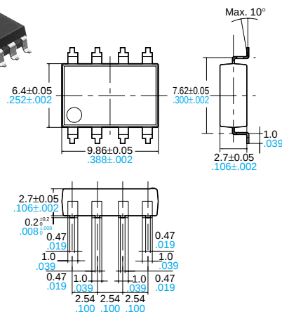
Surface mount terminal type
