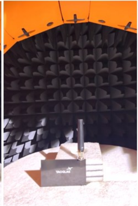
VNA Test Set-up – 15x9cm Ground Plane
