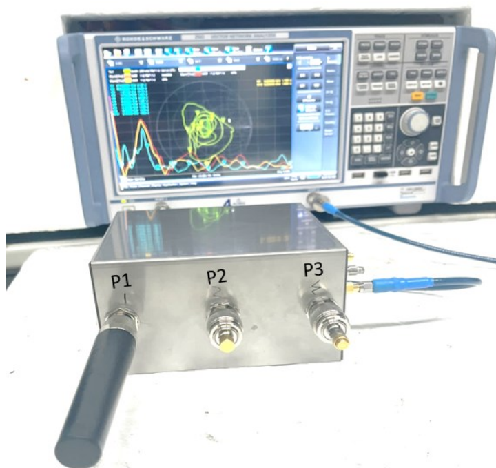
VNA Test Set-up (The Metal box set up above represents a router set up) P1: Port 1 P2: Port 2 P3: Port 3
