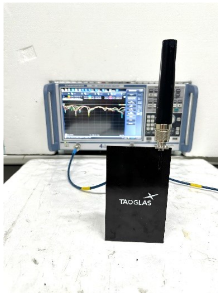
VNA Test Set-up – 9x15cm Ground Plane
