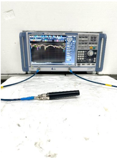
VNA Test Set-up – In Free Space
