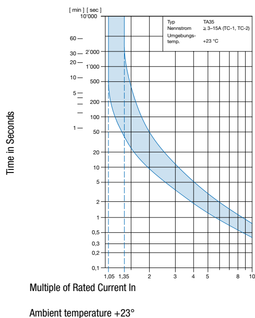
Tripping Characteristics thermal I_n \geq 3 \dots \leq 15A
