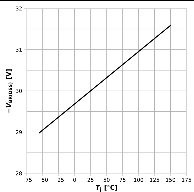
Diagram 30: Drain-source breakdown voltage (p-channel)
