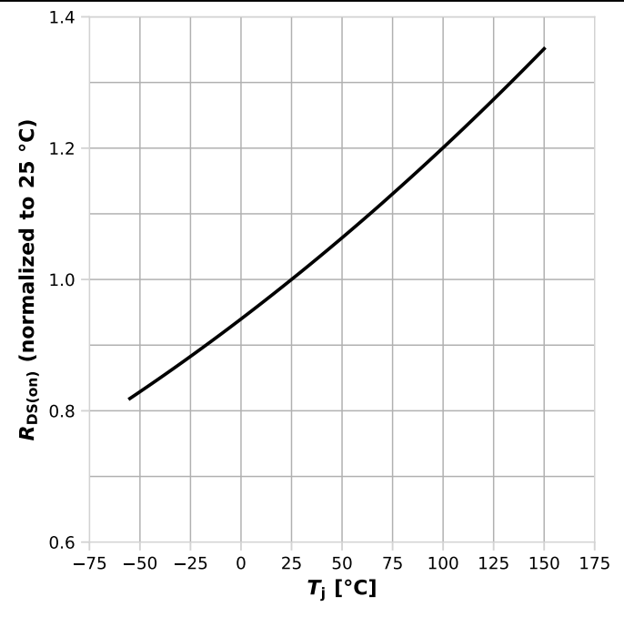
Diagram 24: Normalized drain-source on resistance
