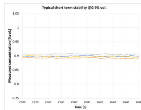
Typical short term precision/Stability @0.9%
