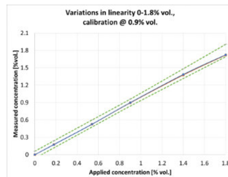
Typical Linearity 0-1.8% Butane
