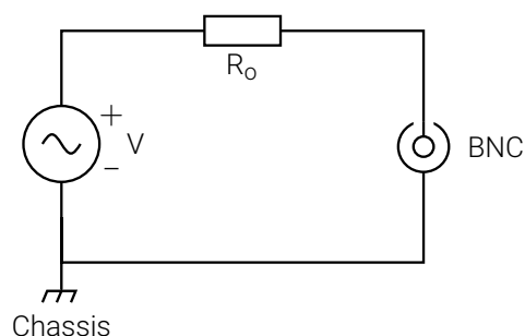
Figure 6: BNC shield and chassis connection
