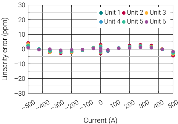
Figure 3: Linearity error of 6 samples
