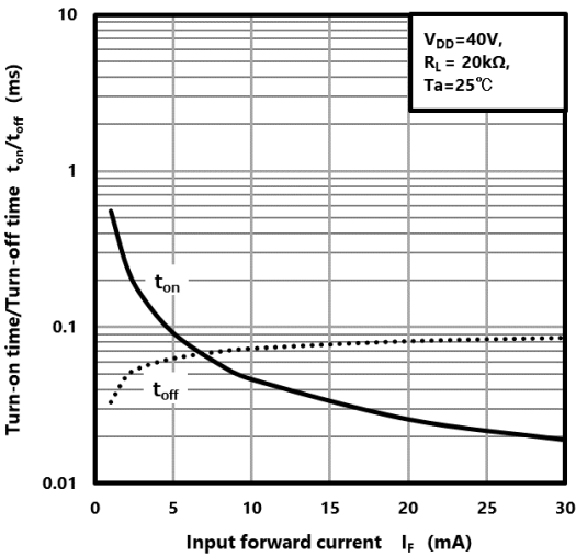
Fig. 12.8 t_{ON}/t_{OFF} - I_F
