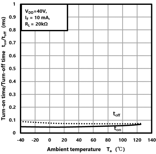
Fig. 12.9 t_{ON}/t_{OFF} - T_a
