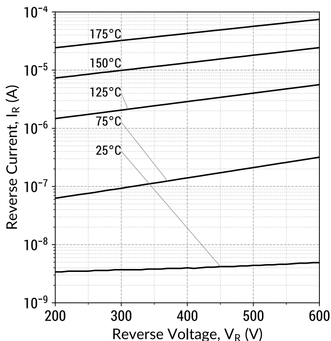
Figure 2: Typical Reverse Characteristics
