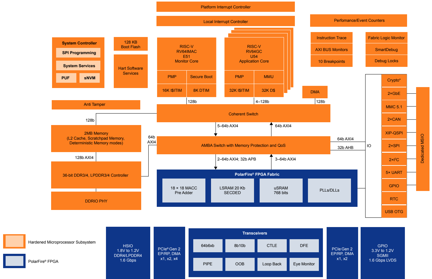
Figure 1-1. Block Diagram
