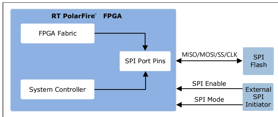
Figure 10-1. SPI Programming Port
