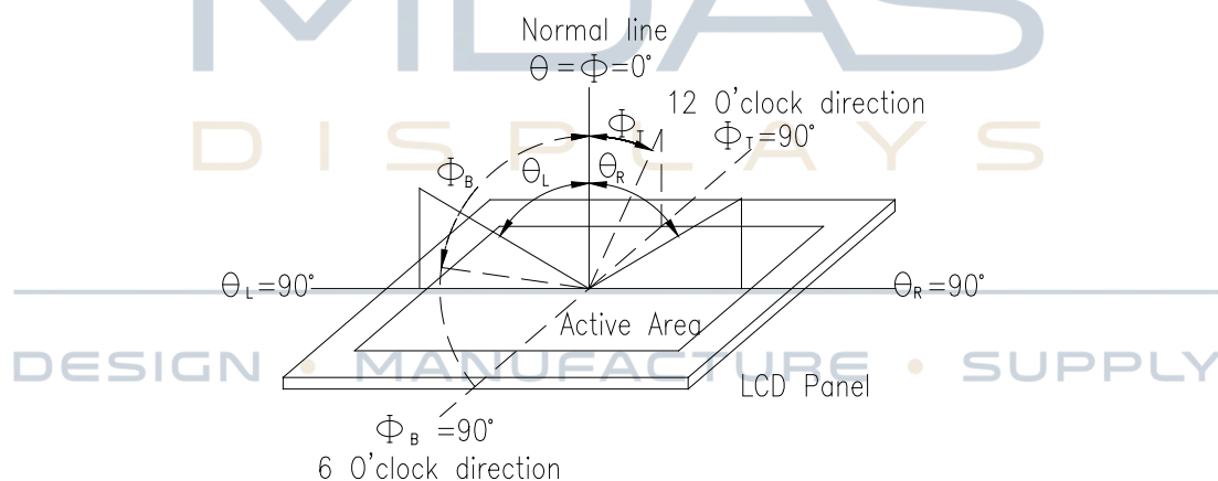
Fig. 8.1. Definition of viewing angle
