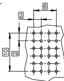
LAYOUT FOR P.C.B (PER 12mm LENGTH)
