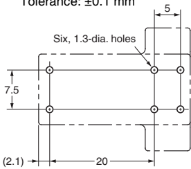
PCB Mounting Holes (Bottom View) Tolerance: ±0.1 mm
