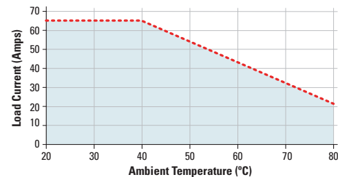
HS072 w/90 Amps single channel SSR
