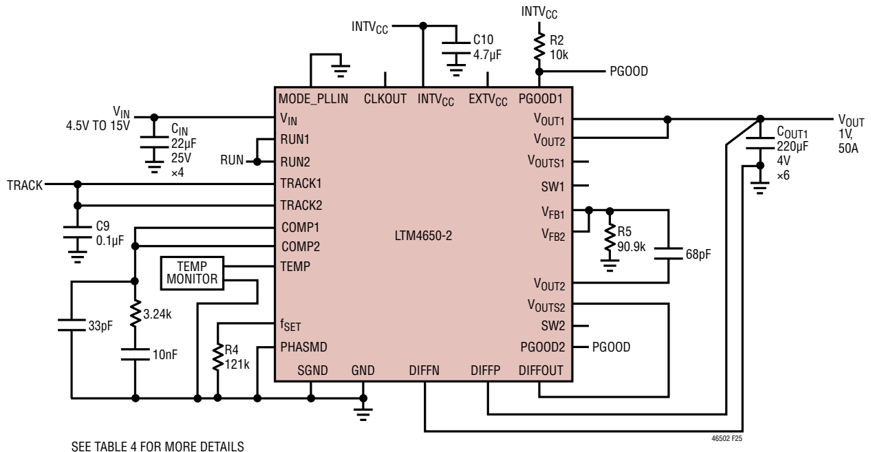
Figure 25. 2-Phase, 1V at 50A Design
