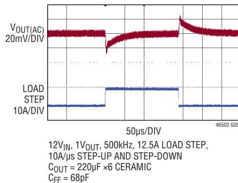
1V Dual-Phase Single Output Load Transient Response
