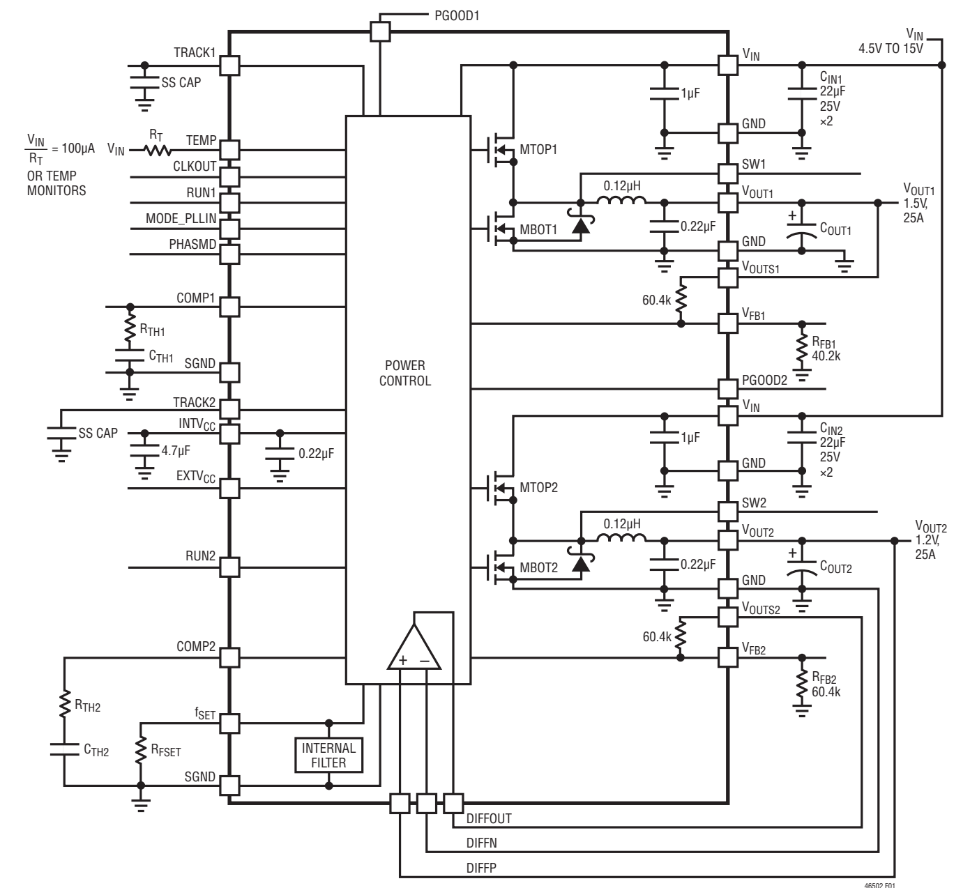
Figure 1. Simplified LTM4650-2 Block Diagram
