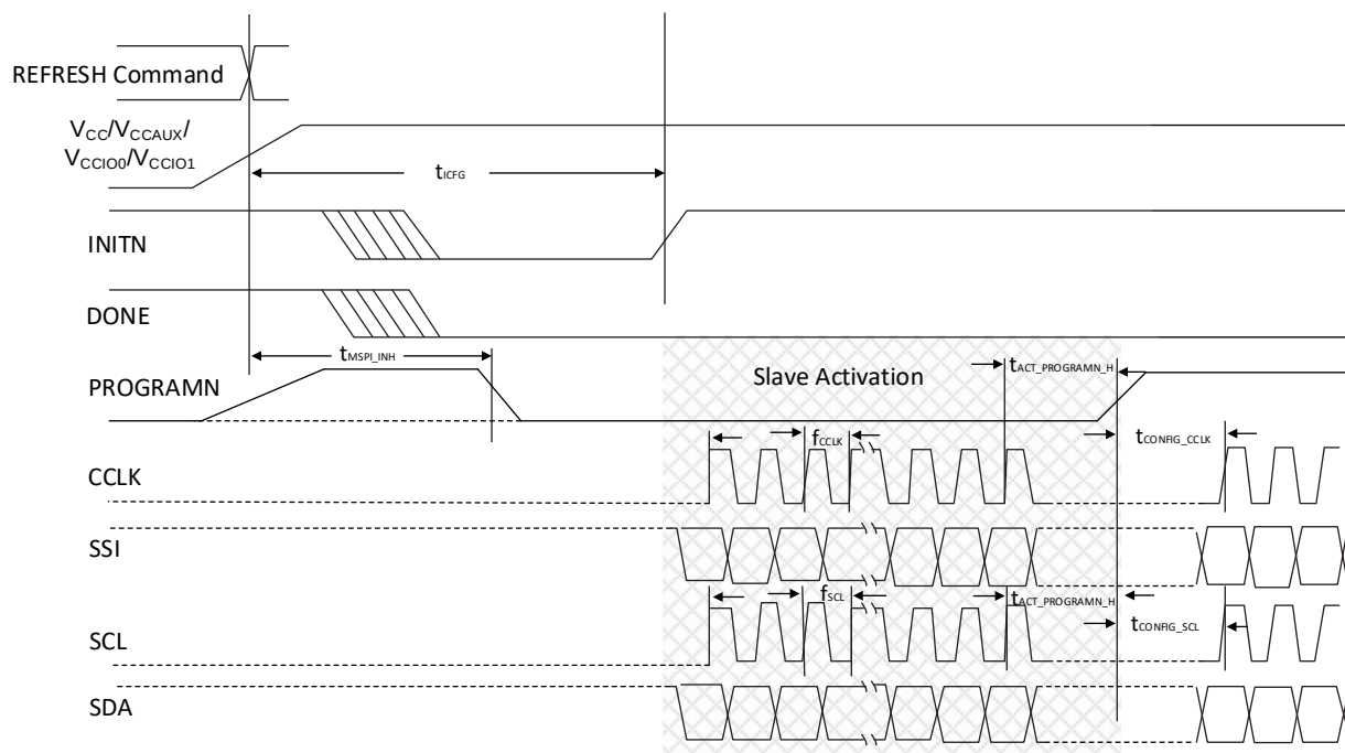
Figure 3.15. Slave SPI/I²C/I³C POR/REFRESH Timing
