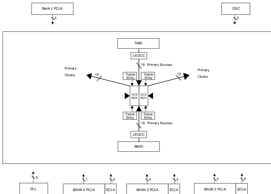
Figure 2.7. Clocking
