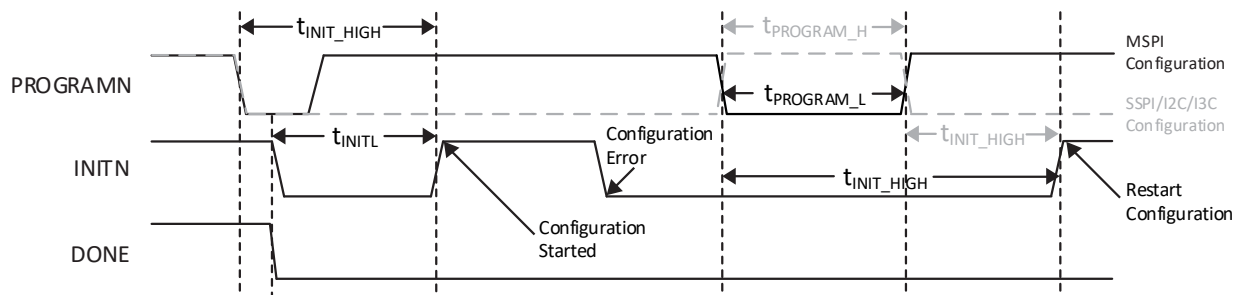
Figure 3.22. Slave SPI/I²C/I3C Wake-Up Timing
