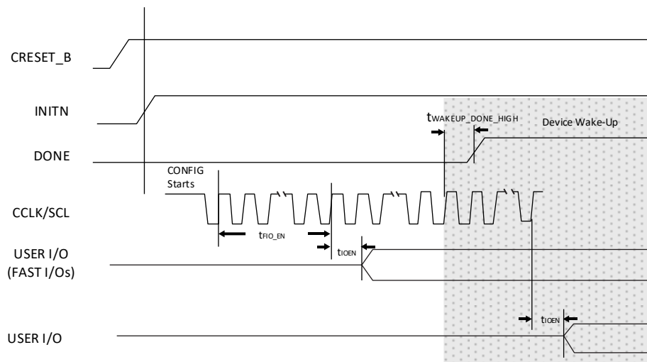
Figure 3.22. Slave SPI/I²C/I3C Wake-Up Timing
