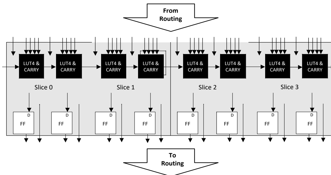
Figure 2.3. PFU Diagram
