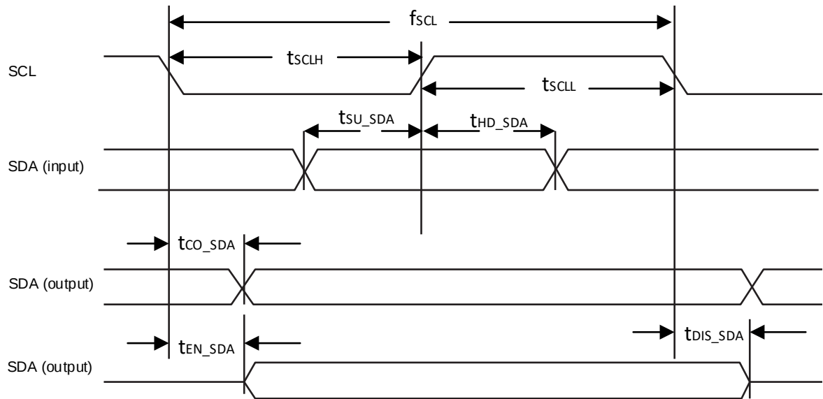
Figure 3.18. I²C /I³C Configuration Timing
