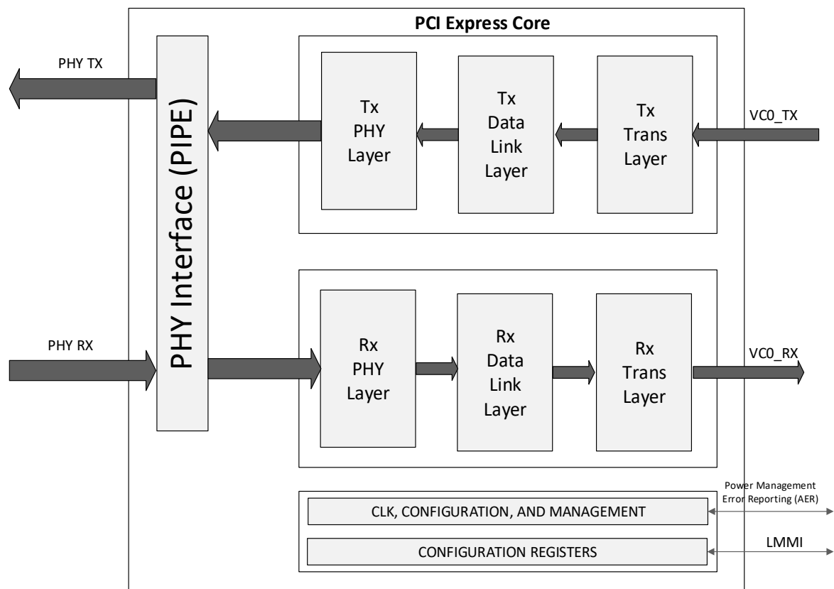
Figure 2.33. PCIe Core
