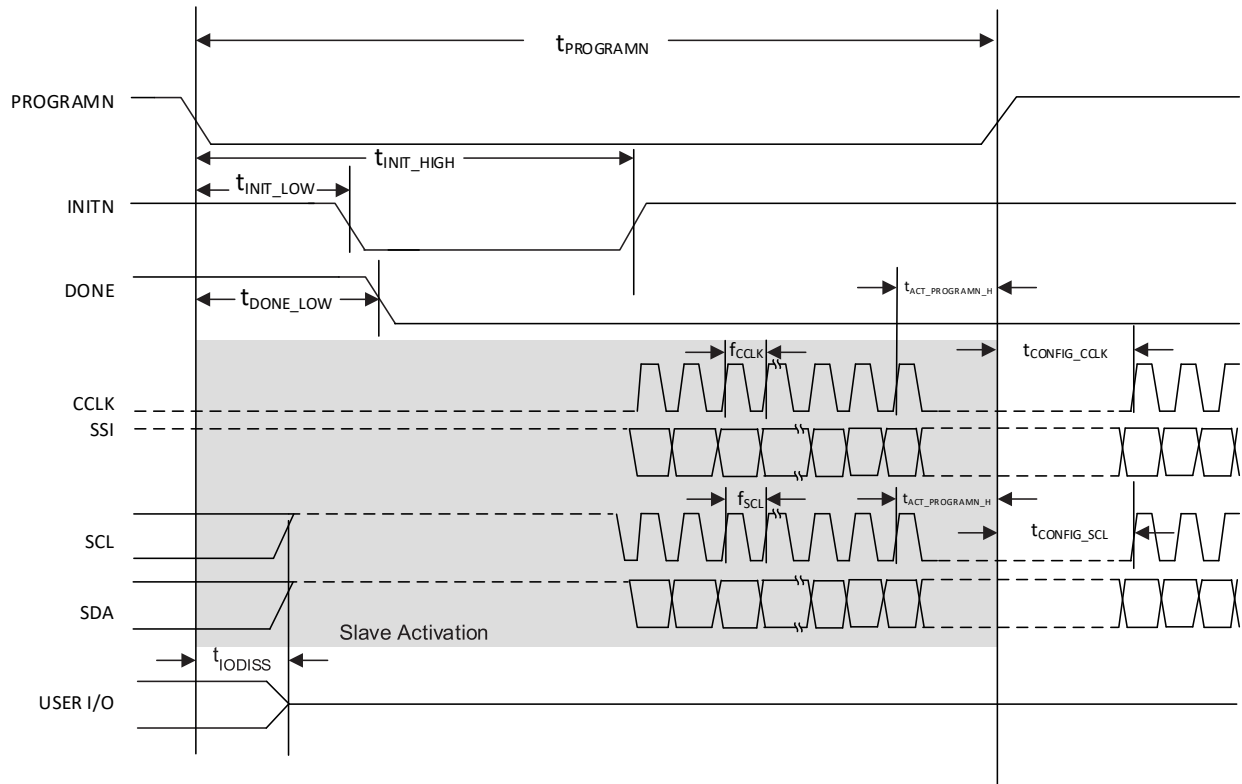
Figure 4.16. Slave SPI/I²C/I³C PROGRAMN Timing
