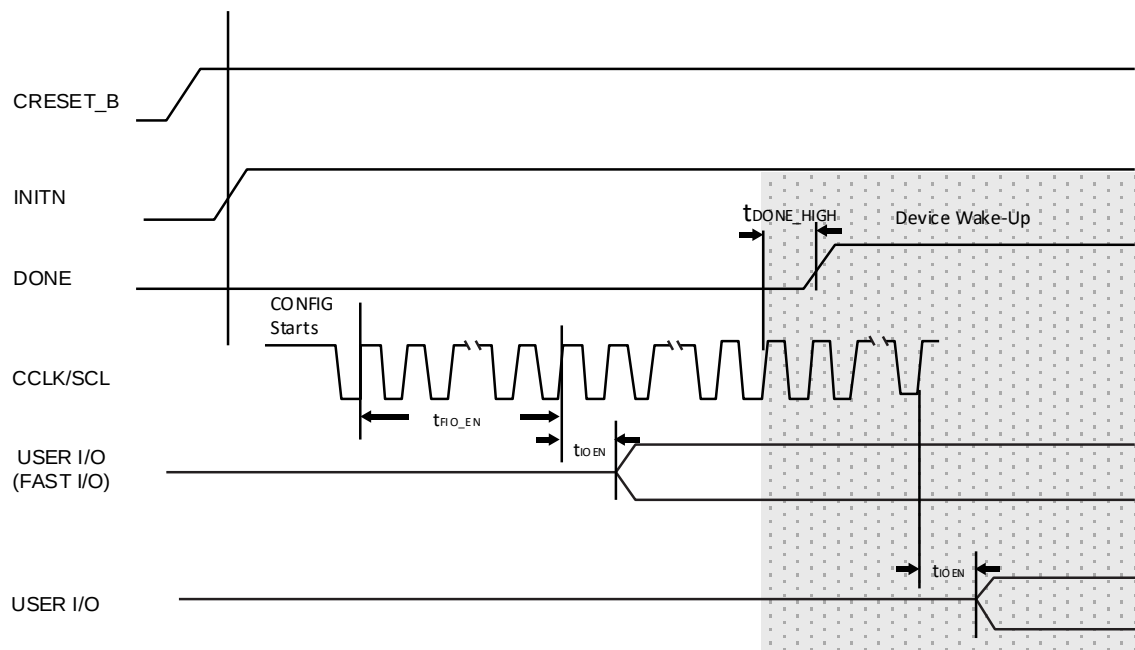
Figure 4.19. Slave SPI/I²C/I³C Wake-Up Timing
