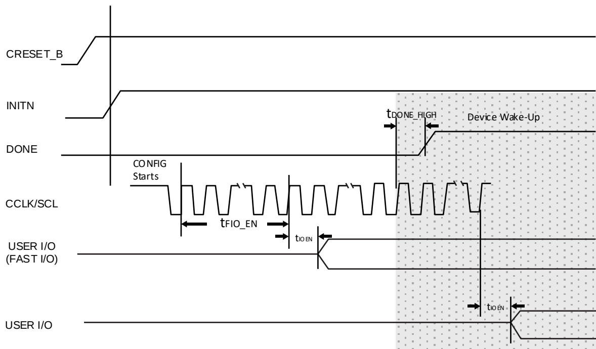
Figure 3.19. Slave SPI/I²C/I³C Wake-Up Timing
