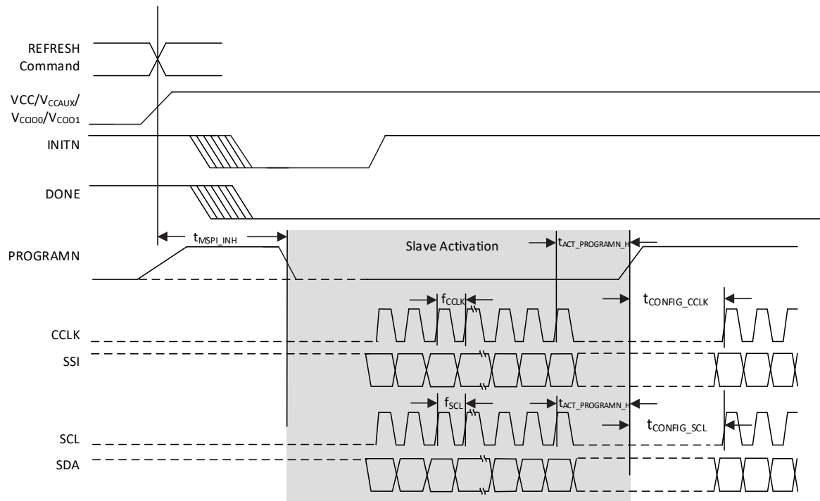
Figure 3.15. Slave SPI/I²C/I3C POR/REFRESH Timing
