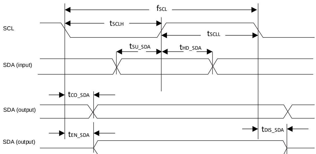
Figure 4.21. I²C/I3C Configuration Timing
