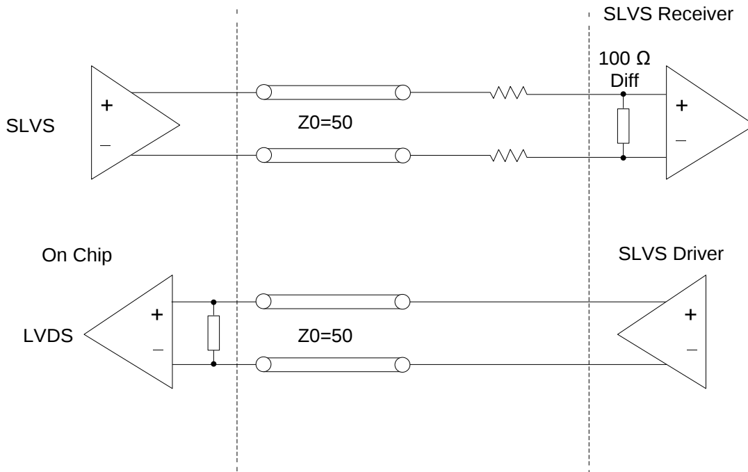
Figure 3.5. SLVS Interface
