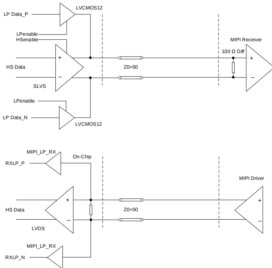
Figure 4.6. MIPI Interface
