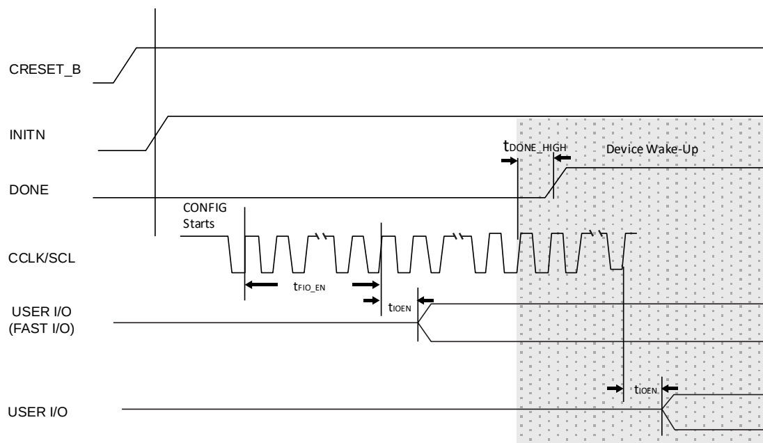
Figure 3.23. Slave SPI/I²C/I³C Wake-Up Timing
