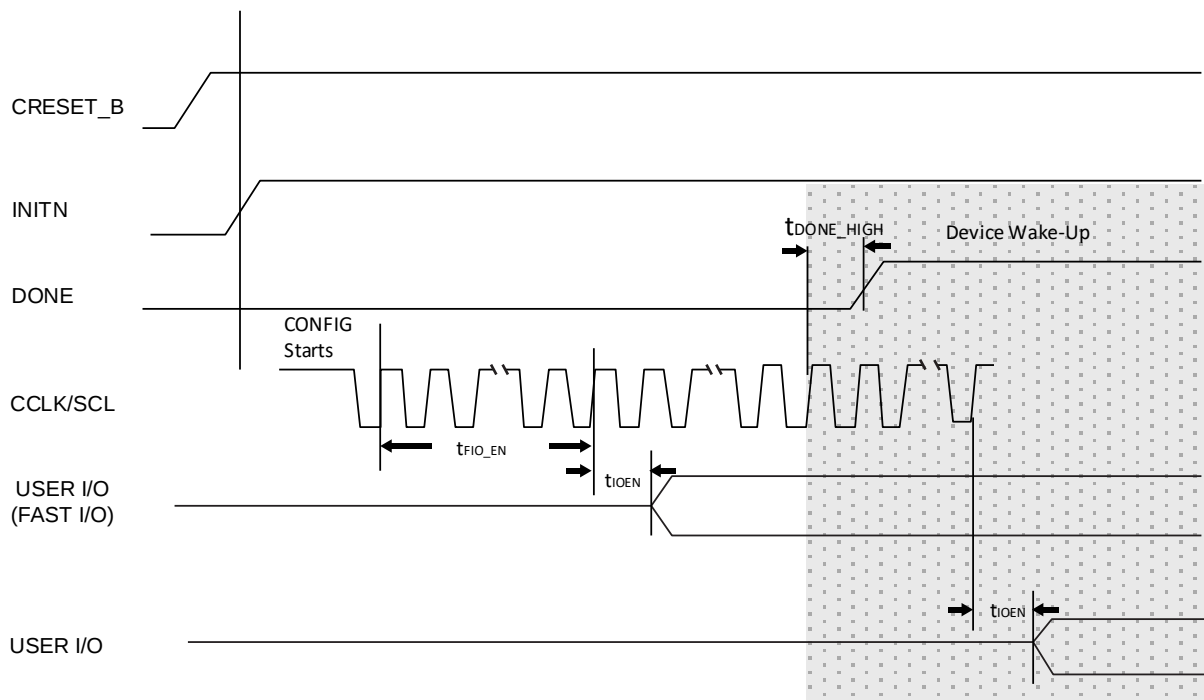
Figure 4.23. Slave SPI/I²C/I³C Wake-Up Timing
