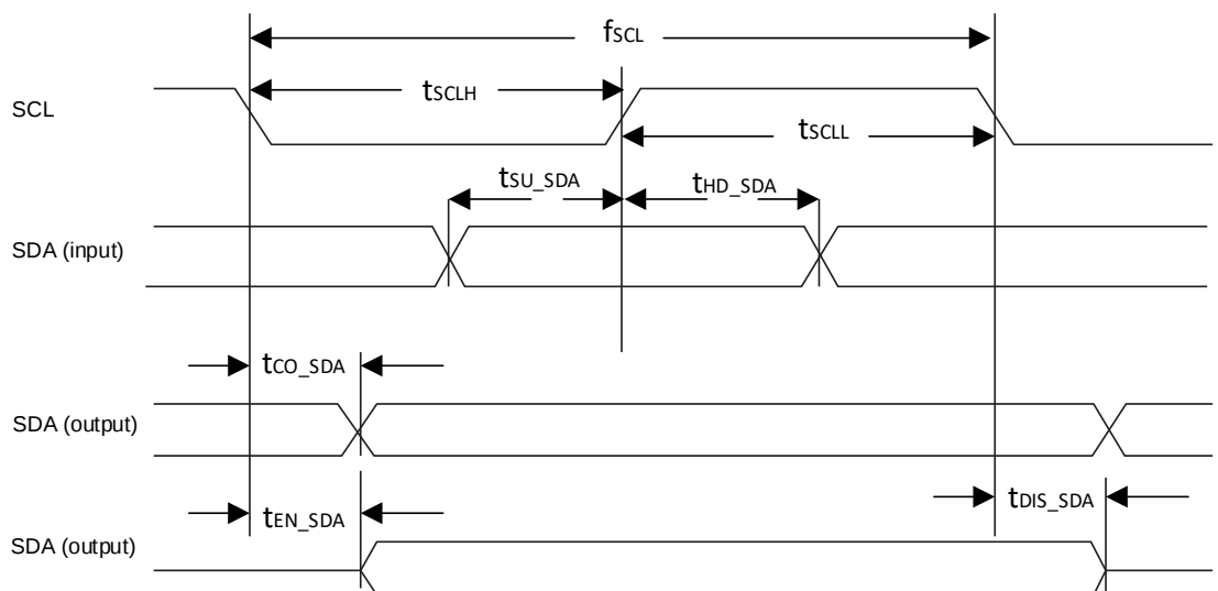
Figure 3.21. I²C/I³C Configuration Timing
