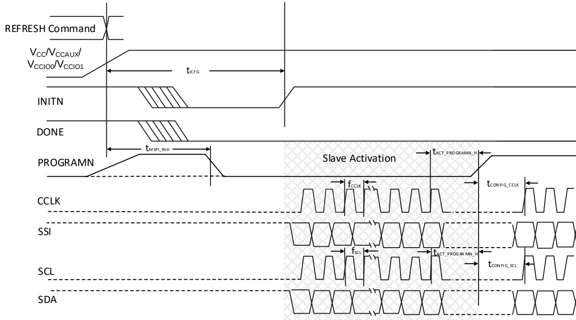
Figure 4.16. Slave SPI/I²C/I³C POR/REFRESH Timing
