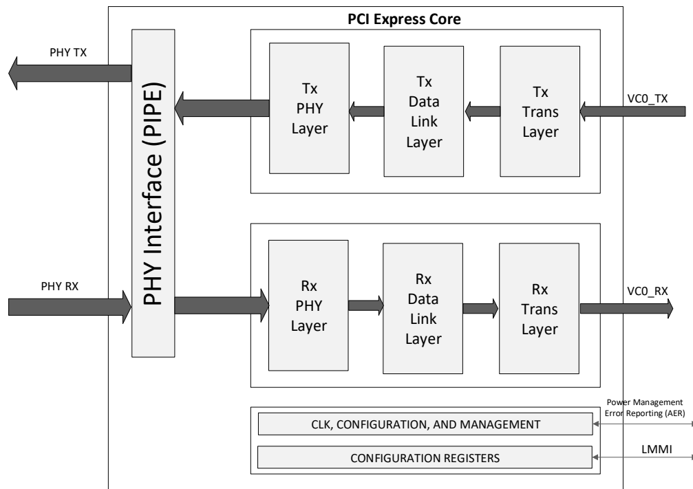
Figure 2.34. PCIe Core
