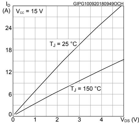
Figure 9. Output characteristics
