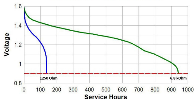
Duracell LR44 Continuous Discharge to 0.9V Cut-off
