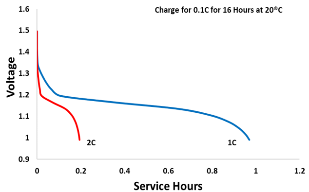
High Rate Discharge- AA Premium
