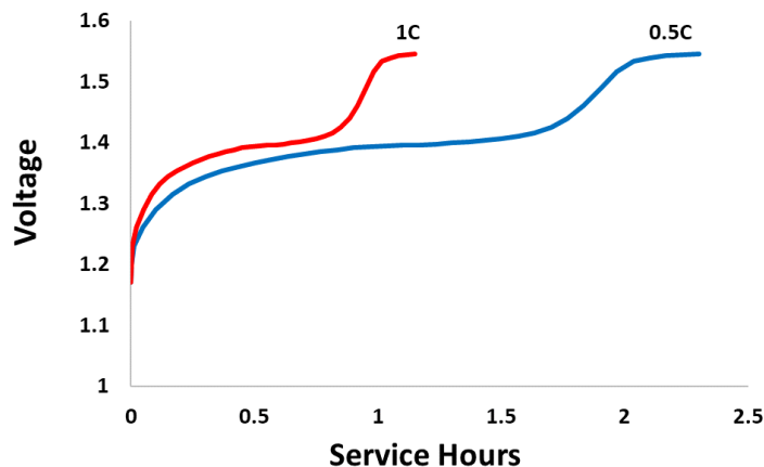
Fast Charge- AA Premium
