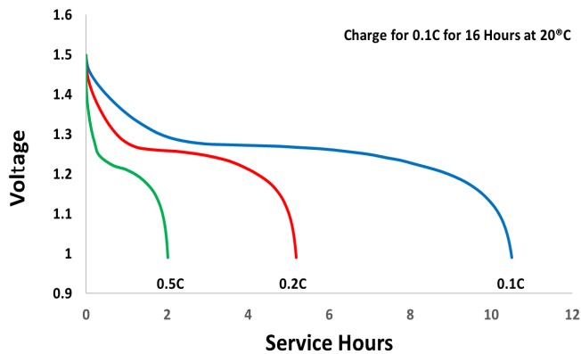
Low Rate Discharge- AA Premium
