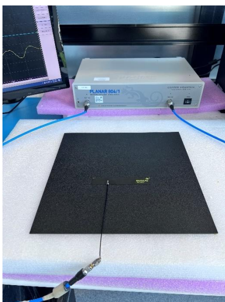
Cable Feed Straight
