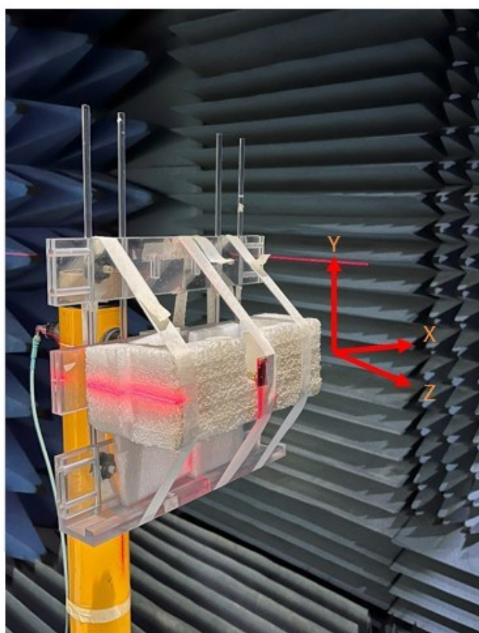
Chamber Test Set-up on a 50x50mm Ground Plane
