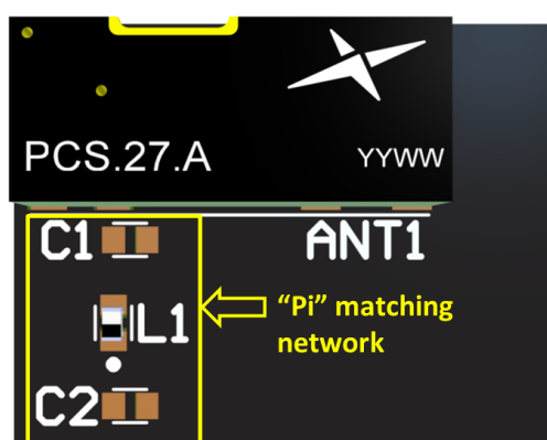
PCS.27.A antenna mounted on a PCB, showing “Pi” matching network.
