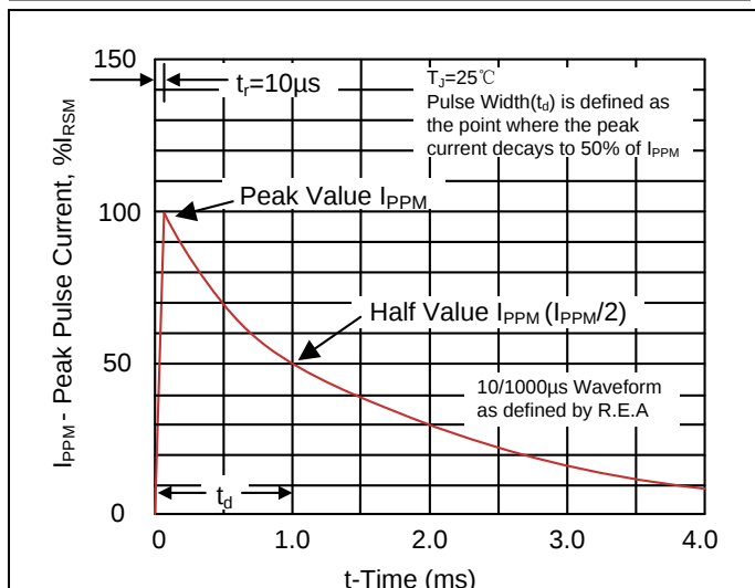
Figure 3. Pulse Waveform
