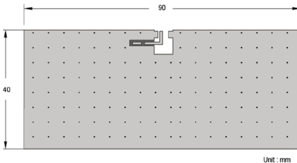
Outlook and dimension of evaluation board
