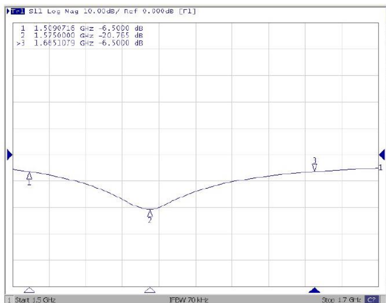
Return loss
