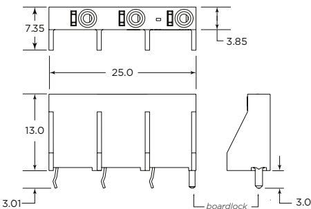
position in-line screwless wire connector
