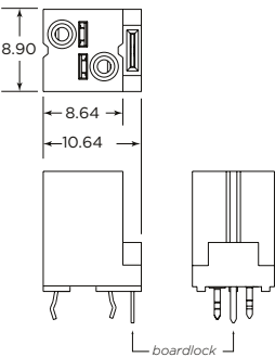
2 position screwless wire connector4
