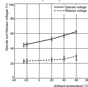
Ambient Temperature vs. Operate and Release Voltage G7L-1A VAC (60 Hz)
