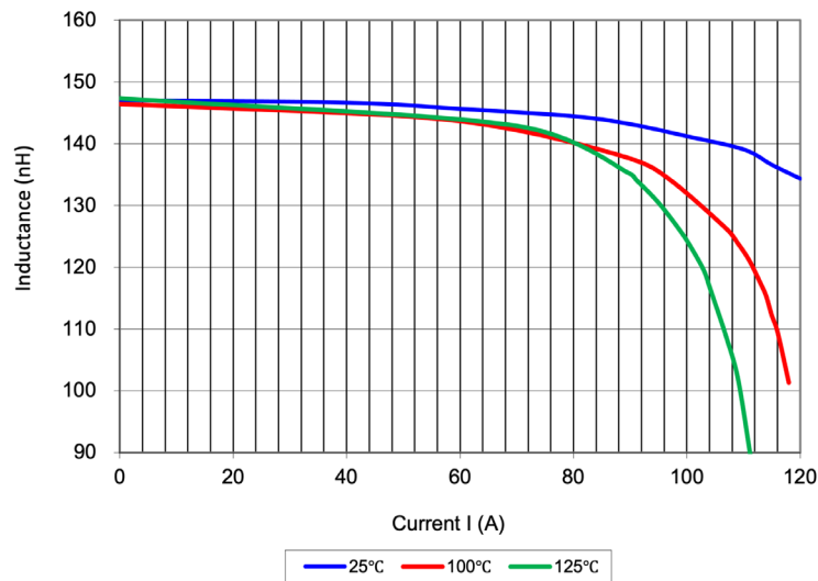
PA5615.800HLT, L vs I Curve
