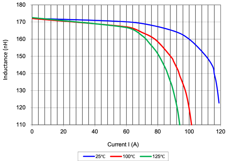
PGL6395.121HLT, L vs I Curve
