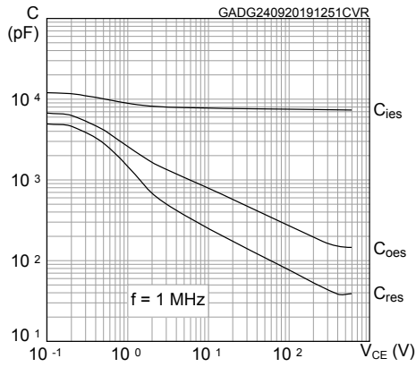
Figure 13. Capacitance variations
