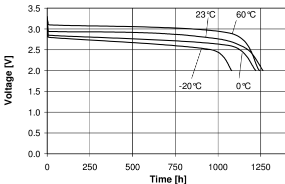
Temperature performance Load 12kΩ
