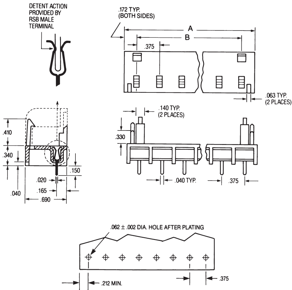
Recommended PCB Hole Pattern
