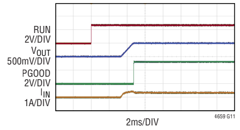
Start-Up with Prebiased Output
