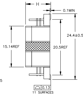
FINAL OUTLINE
