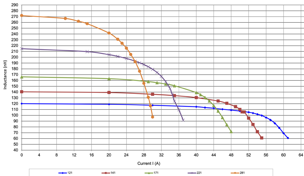
PGL6478.XXXHL L vs I curve 125°C
