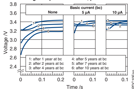
Voltage Response at +25 °C, pulse: 10 mA
