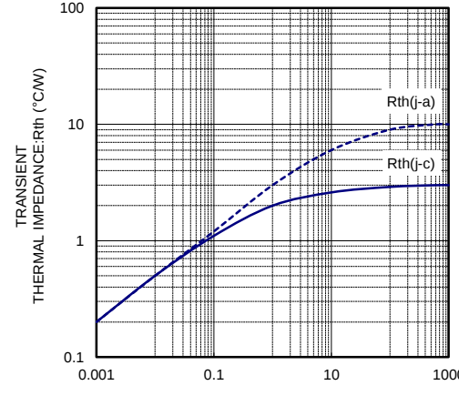
R_th-t CHARACTERISTICS
