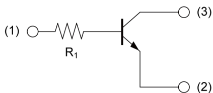
(1) BASE (2) EMITTER (3) COLLECTOR
