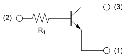
(1) EMITTER (2) BASE (3) COLLECTOR
