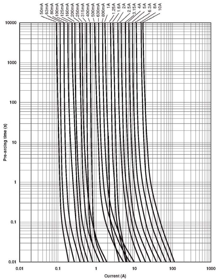
Time - Current Curve
