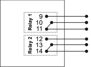
RELAY OUTPUTS
