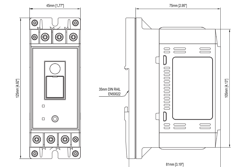
Fig. 1 RSBT..V11 HP versions
