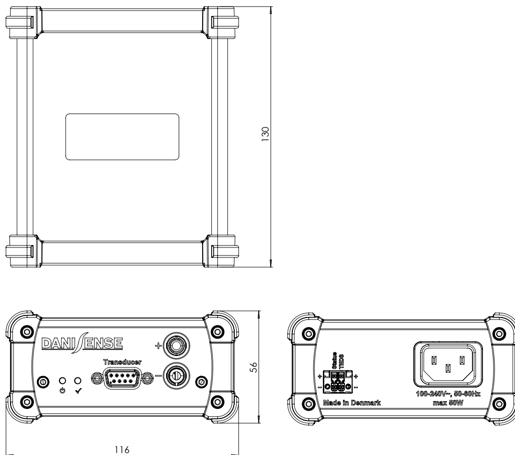
Figure 3: Box dimensions
