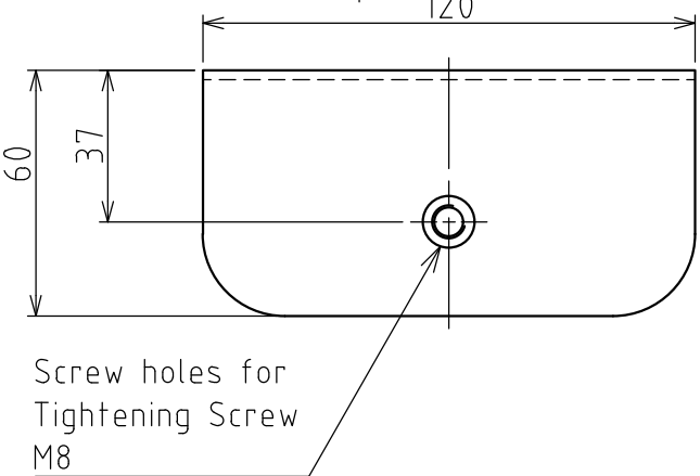
External Dimensions (Partition Mounting Bracket)
