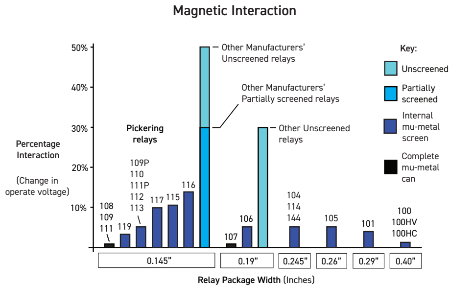
This chart demonstrates the percentage changes in operate voltage due to magnetic interaction depending on the level of magnetic screening offered from the relay package. For more information on magnetic interaction click here .
